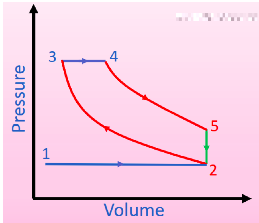
Figure 73.5: Blue: Isobaric, Green: Isochoric, Red: Adiabatic
