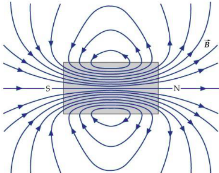
Figure 32.1: Magnetic Field Lines Around a Bar Magnetic
