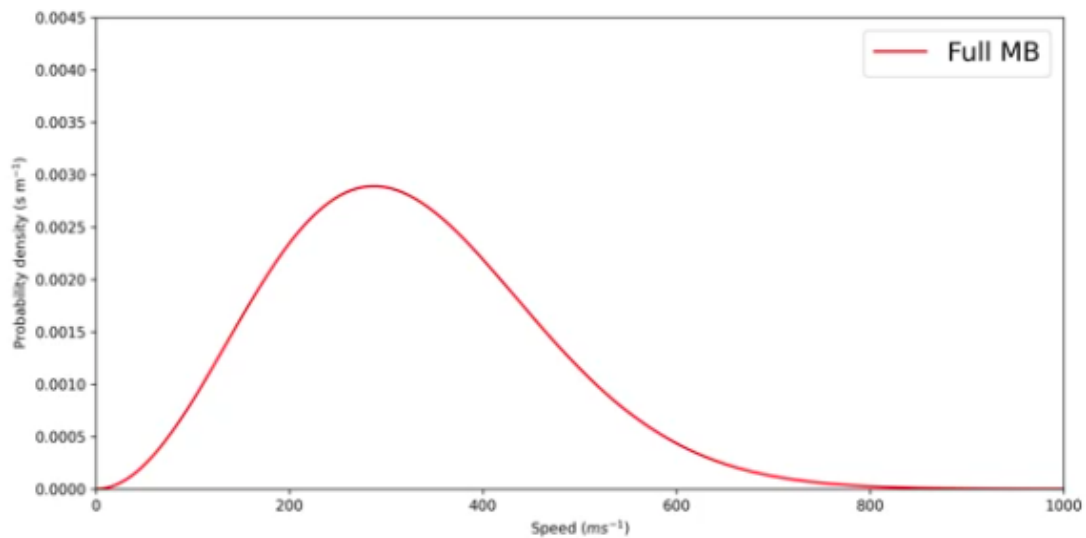
Figure 80.1: Maxwell-Boltzmann Distribution for T = 10\text{K} . Note that the value is approaching zero for v \approx 1000 , let alone c .
