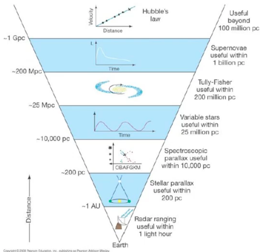
Figure 43.2: The Cosmic Distance Ladder
