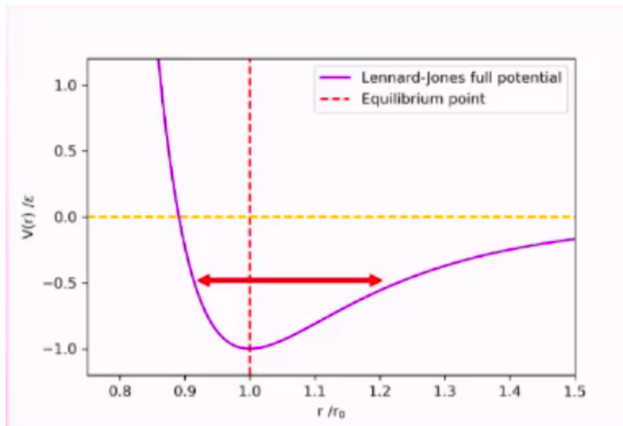
Figure 69.2: LJ Potential
